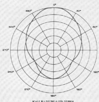
FIGURE 4 Polar Pattern, 700–1300 Hz Sweep Square Wave (on typical 8 in. diameter reentrant horn)
