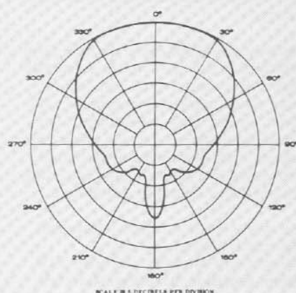
FIGURE 5 Polar Pattern, 700–1300 Hz Sweep Square Wave (FR150 horn)
